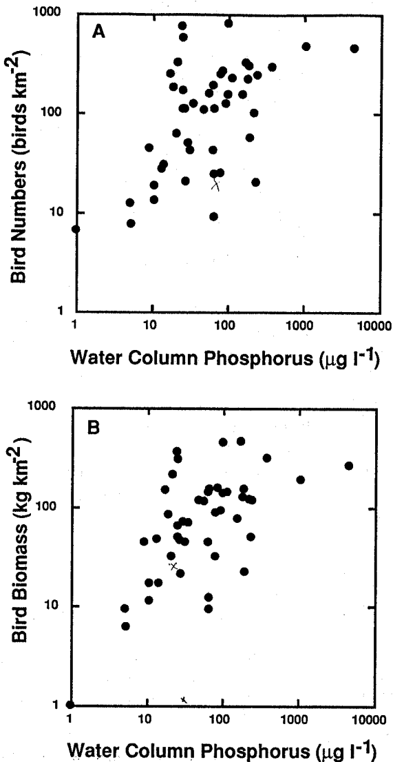
Fig. 1. Relation between annual average bird numbers (A, birds \text{km}^{-2} ) and biomass (B, \text{kg km}^{-2} ) and water column phosphorus concentration (WCP, \mu\text{g l}^{-1} ) for 46 Florida lakes. WCP values are calculated by adding the phosphorus incorporated in aquatic macrophyte and epiphytic algae tissue to the measured total phosphorus concentration according to the methods of Canfield et al. (1983).
